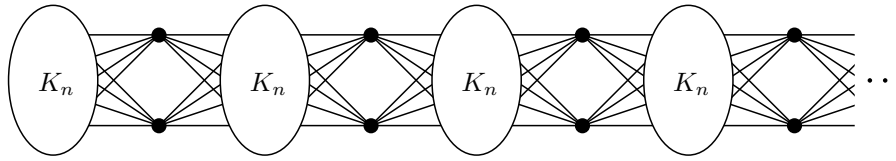
Figure 1: Complete graphs glued together at separators of size two along a ray. The method of Dunwoody and Krön gives a tree-decomposition of this graph along an end whose separators have size two.
