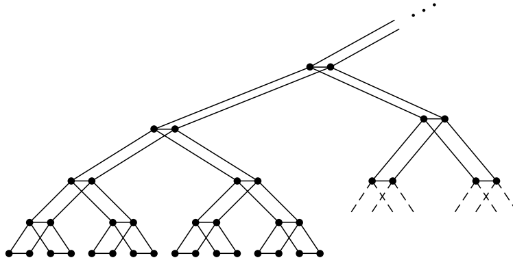
Figure 2: The product of the canopy tree with K_1 . This graph has a tree decomposition whose decomposition tree is the canopy tree.
