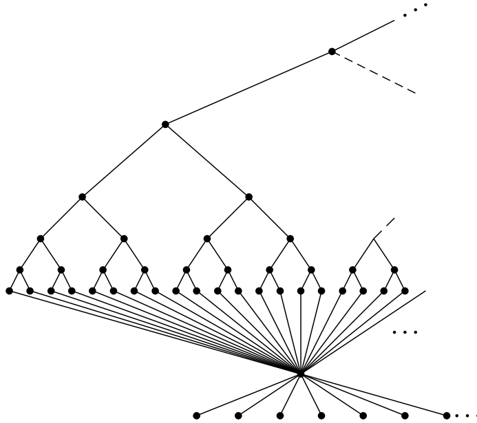
Figure 3: A graph with no \text{Aut}(G) -invariant tree-decomposition of finite adhesion.
